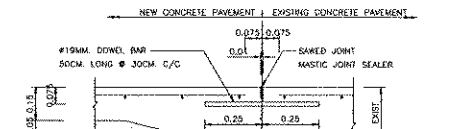
DETAIL OF LONGITUDINAL JOINT
