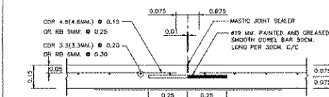
DETAILS OF CONTRACTION JOINT
