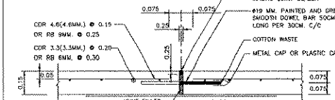
DETAILS OF EXPANSION JOINT
