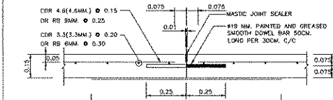
DETAILS OF CONSTRUCTION JOINT
